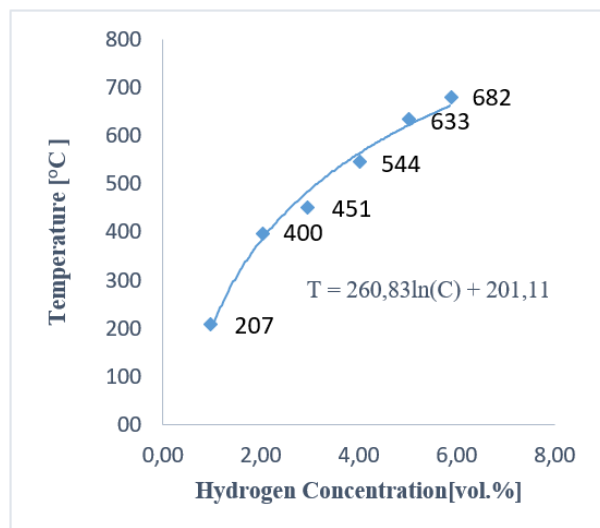
Figure 13 Correlation between PAR inlet concentration and maximum catalysts temperature
