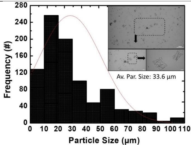
Fig. 1. Particle size distribution histogram of perlite (inset: optical microscope images of perlite at different magnifications. Scale bars are 100, 50 and 10 \mu\text{m} , respectively)
