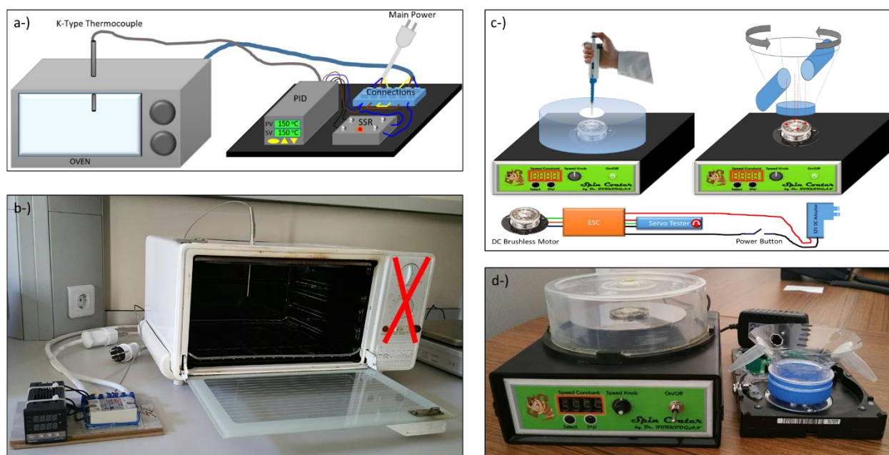
Figure 1. Schematic illustrations and real color images of homemade laboratory oven (a-b), spin coater and centrifuge (c-d). Bottom part of (c) shows the electronic control diagram of spin coater, centrifuge and magnetic stirrer.
