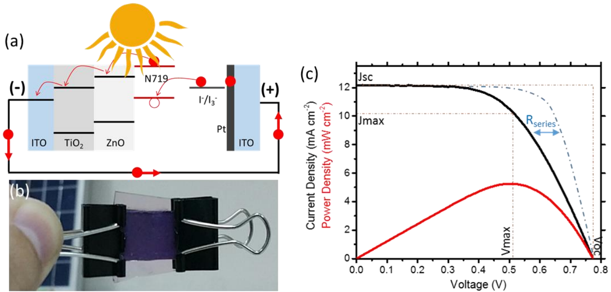
Figure 4. (a) Schematic illustration of TiO 2 /ZnO hybrid structure based DSSC w/ Pt counter electrode (b) Real color image of the constructed cell. (c) JV and PV curves of the corresponding solar cell with the indication of some important parameters.
