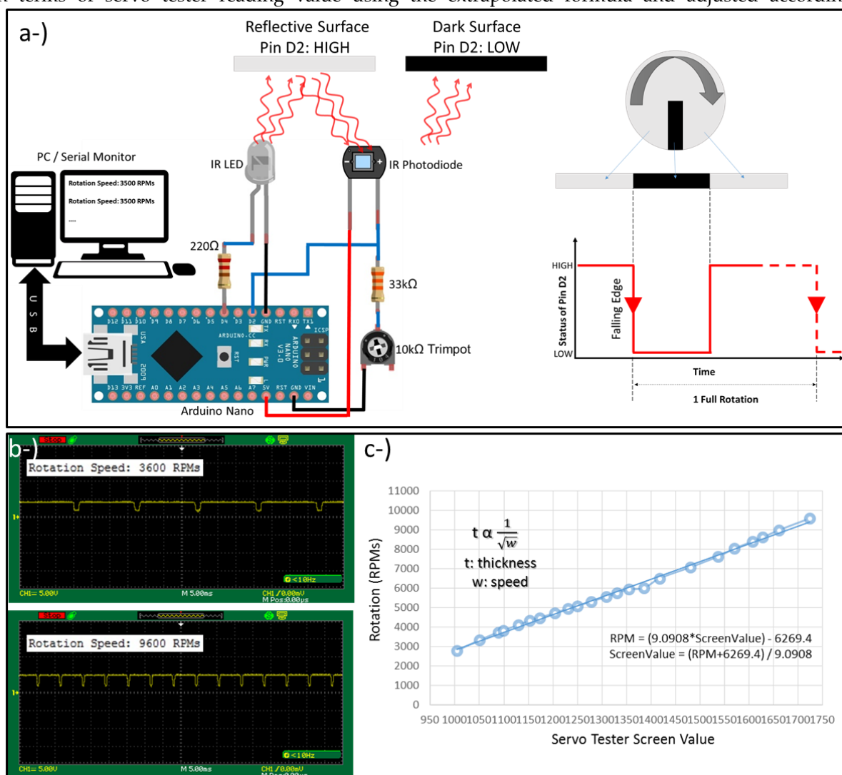
Figure 2. (a) Schematic of the optical tachometer with the illustration of photodetectors's signal as PD facing the reflective and dark surfaces on the spinning plane. (b) Pin D2's signal input taken from the Oscilloscope screen when the spin coater rotates at 3600rpms and 9600rpms, respectively. Insets with white background show the serial monitor output. (c) Rotation speed of the spin coater as a function of servo tester's set value.
