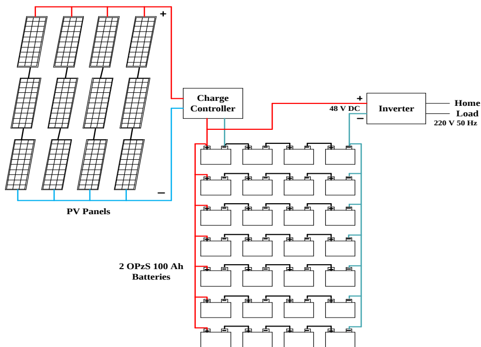
Figure 1. The schematic of the stand-alone PV system
