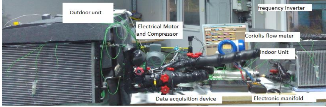
Figure 2. The photo of experimental MAC system and measuring devices
