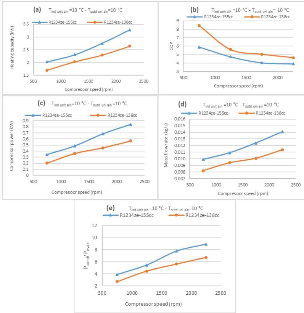
Figure 5. Variations of the performance characteristics as a function of compressor speed and compressor volume under the system using R1234ze(E) a) Heating capacity b) COP c) Compressor power d) Mass flow rate e) P_{cond}/P_{evap}
