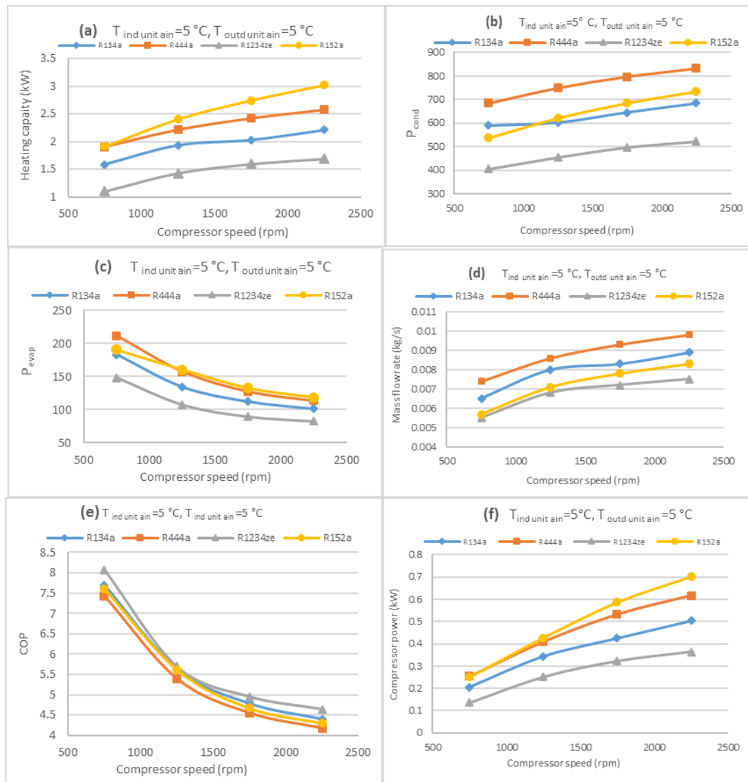
Figure 3. Variations of the performance characteristics with compressor speeds a) Heating capacity b) P_{\text{cond}} c) P_{\text{evap}} d) Mass flow rate e) COP f) Compressor power
