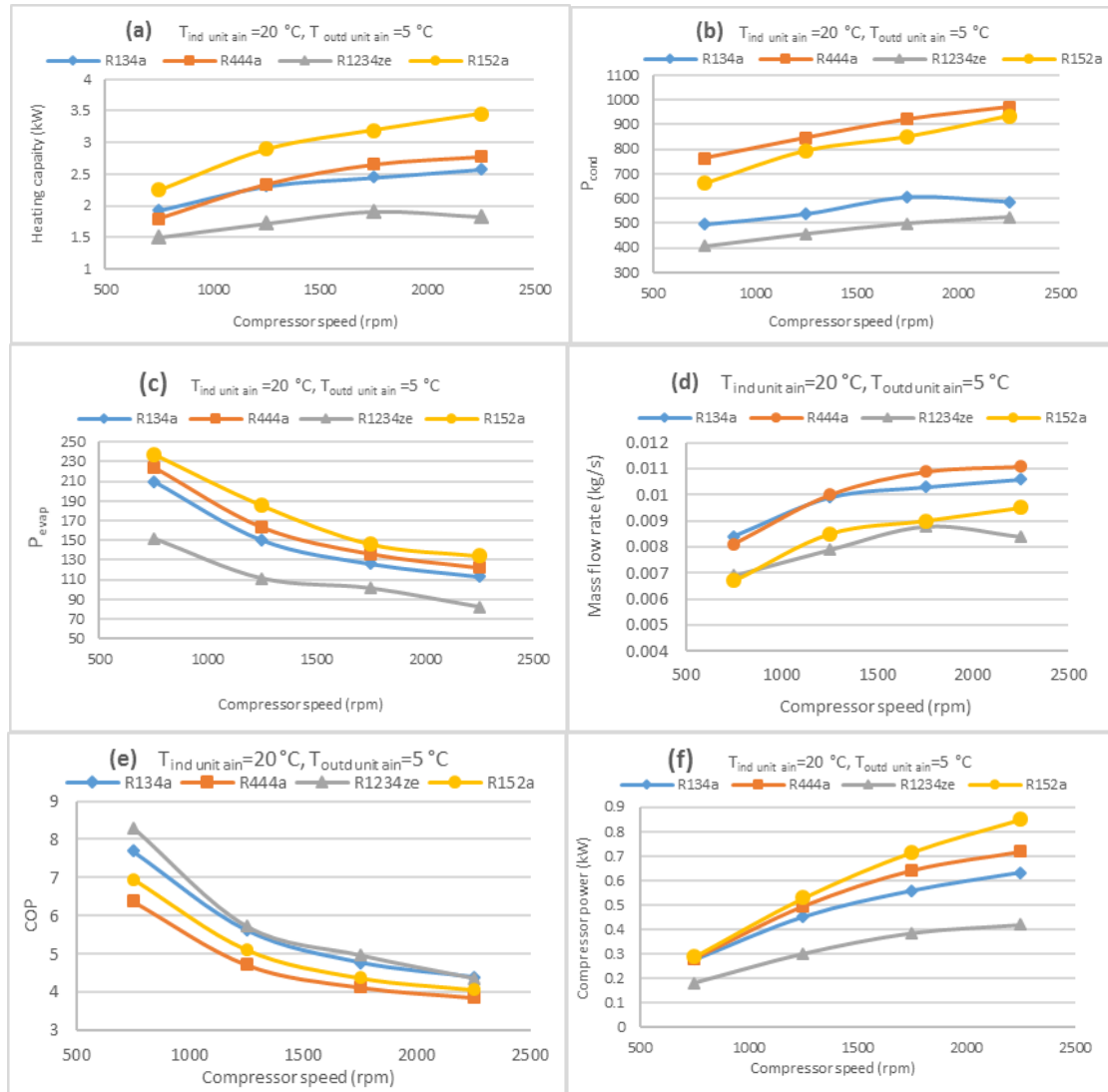
Figure 4. Variations of the performance characteristics with compressor speeds a) Heating capacity b) P_{cond} c) P_{evap} d) Mass flow rate e) COP f) Compressor power
