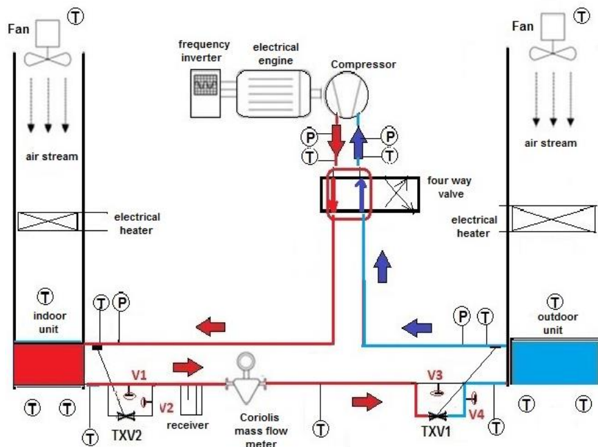
Figure 1. Schematic diagram of MAC system in heating mode
