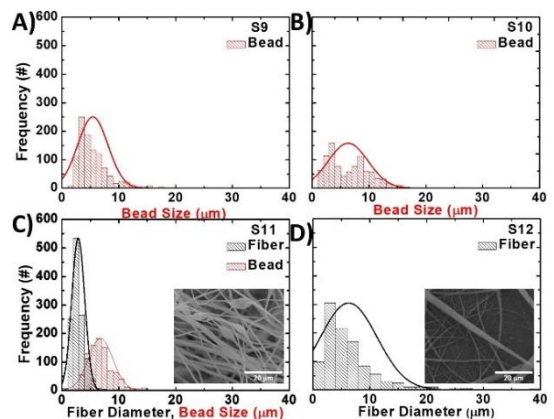
Figure 12. Fiber diameter and/or bead size distributions of a) S9, b) S10, c) S11, and d) S12
